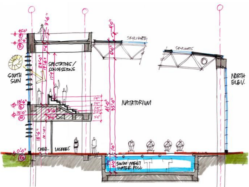
BUILDING SECTION
